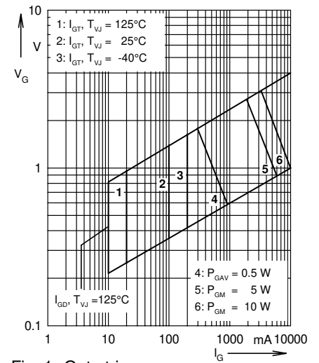
Fig. 1 Gate trigger range
